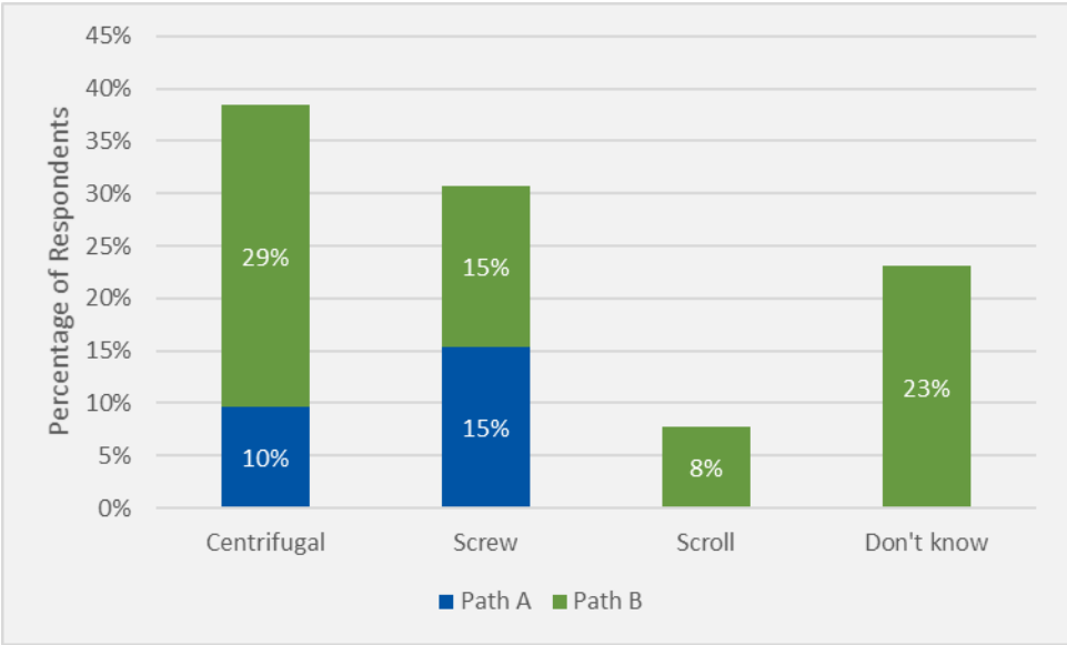
Figure 8. Installed Chiller Types
